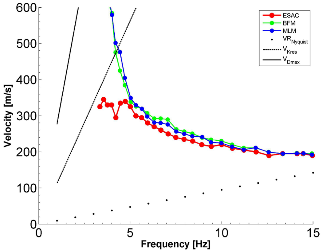
Fig. 14.13 Phase velocity dispersion curves obtained by ESAC (reds line), BFM (green line) and MLM (blue line) analysis. The dotted line indicate the theoretical aliasing limit calculated as 4 f d_{min} , where d_{min} is the minimum interstation distance. The factor 4 is used instead of the generally used factor 2, because the minimum distance in the array is appearing only once. The dashed gray line indicates the lower frequency threshold of the analysis based on 2\pi f \Delta k where \Delta k is calculated as the half-width of the main peak in the array response function. The continuous line indicates the lower frequency threshold of the analysis based on the equation 3 f d_{max} , where d_{max} is the maximum interstation distance in the array
